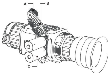
FIGURE 2-1. BATTERY INSTALLATION
